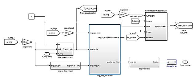
Figure 8: Internal Combustion Engine (ICE) Block Diagram.
