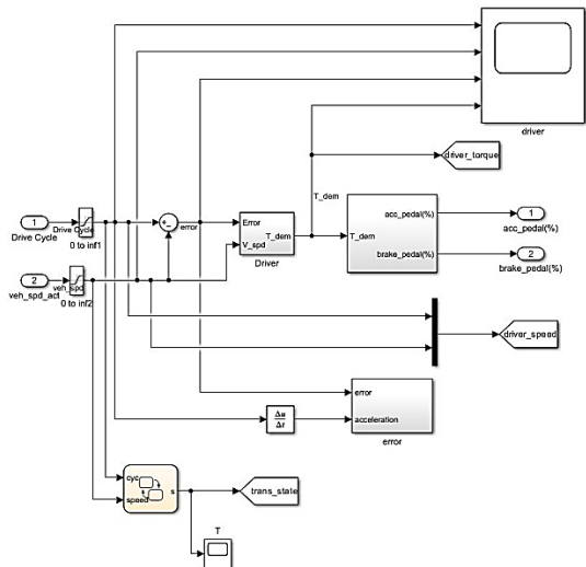
Figure 7: Driver block structure.
