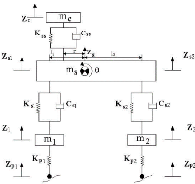
Figure 2. Vehicle vibration model [10, 12].
