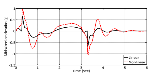
Figure 24. Middle wheel acceleration
