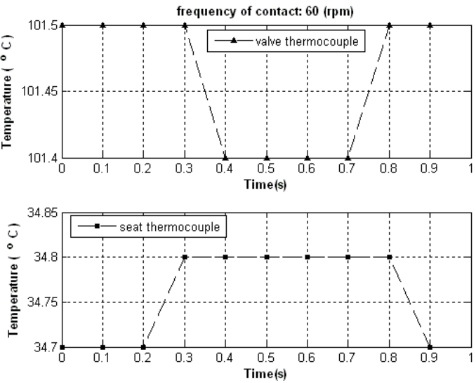
Fig6. Temperature distribution at the nearest thermocouples to the interface for the speed of 60 rpm
