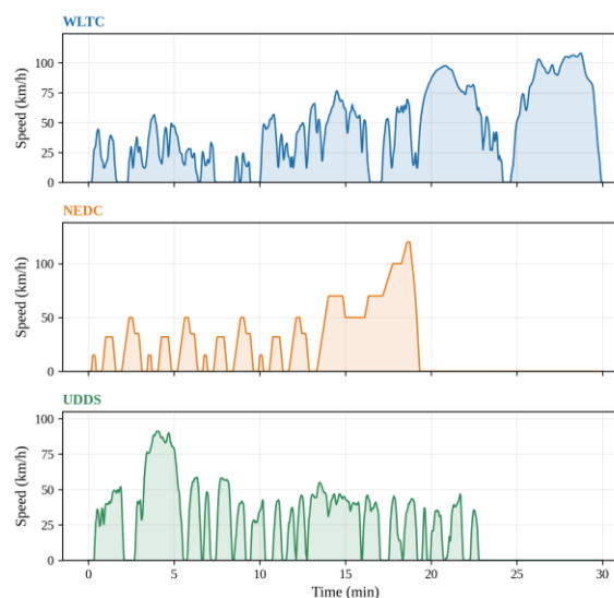
Figure 3: Vehicle speed profiles for the three simulated driving cycles: (top) WLTC, (middle) NEDC, (bottom) UDSS.
