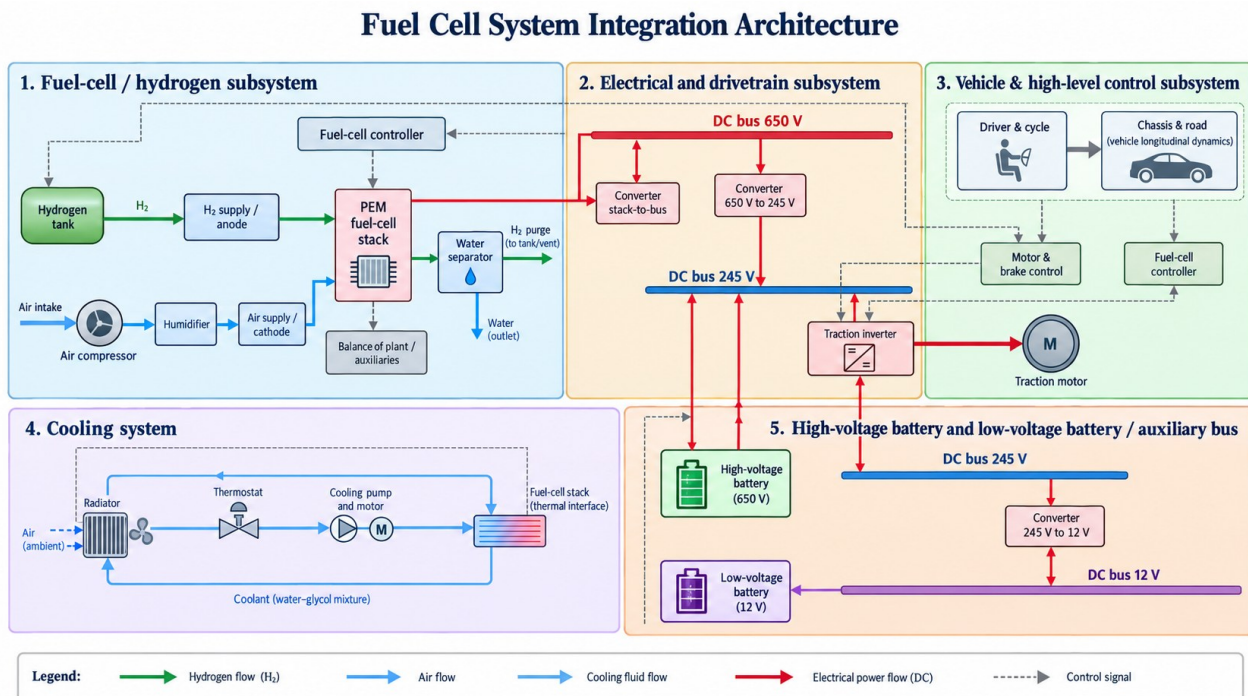
Figure 1: Schematic architecture of the simulated fuel-cell/battery hybrid powertrain and its principal power- and signal-flow paths.
