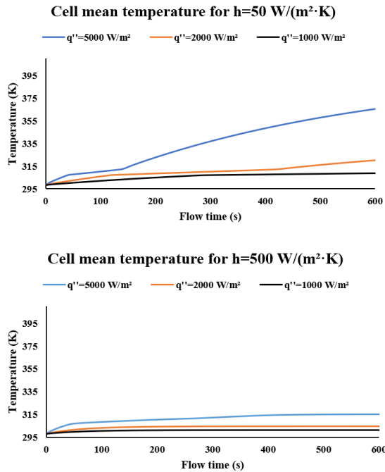
Figure 4: The cell mean temperature for heat transfer coefficients of h=50 and h=500 W/(m 2 ·K)
