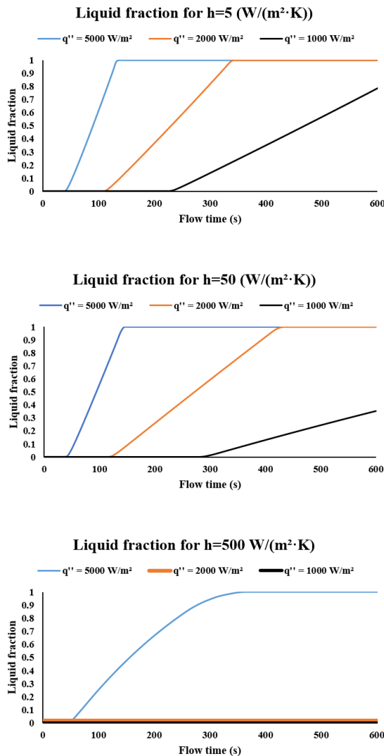
Figure 8: Liquid fraction of the PCM layers in the composite for heat transfer coefficients of h=5 , h=50 and h=500 \text{ W/(m}^2 \cdot \text{K)}
