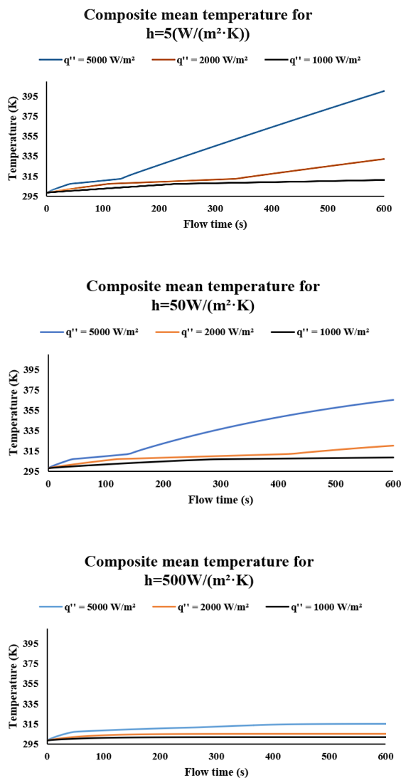
Figure 5: The average temperature of the composite for heat transfer coefficients of h=5 , h=50 and h=500 \text{ W/(m}^2\cdot\text{K)}
