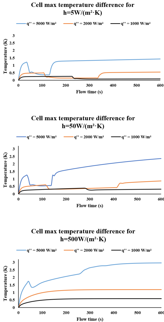
Figure 6: The maximum temperature difference between the cell and the composite for heat transfer coefficients of h=5 , h=50 and h=500 \text{ W/(m}^2 \cdot \text{K)}
