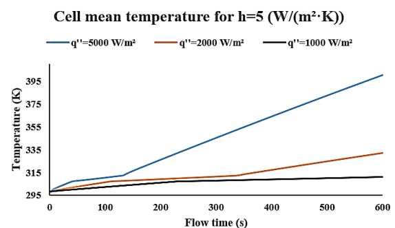
Figure 3: The cell mean temperature for heat transfer coefficients of h=5 \text{ W/(m}^2\cdot\text{K)}
