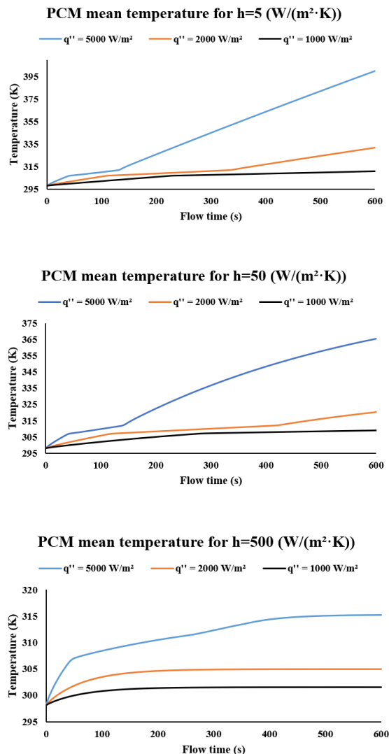
Figure 7: The average temperature of the PCM layers in the composite for heat transfer coefficients of h=5 , h=50 and h=500 W/(m²·K)
