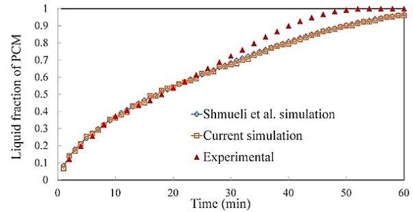
Figure 2: Validation of the numerical method with the experimental data [16]; the results of another numerical simulation [15] are also illustrated.
