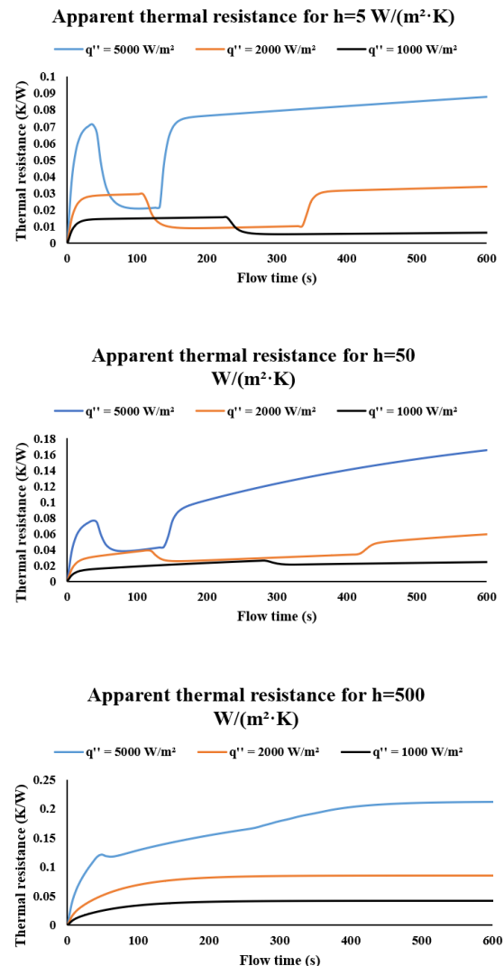
Figure 9: Apparent thermal resistance of the heat pipe for heat transfer coefficients of h=5 , h=50 and h=500 \text{ W/(m}^2 \cdot \text{K)}
