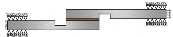
Figure 2: Applied boundary conditions and loading on the SLJ model.
