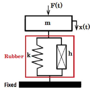
Figure 1: An equivalent SDOF dynamic model of the PREM
