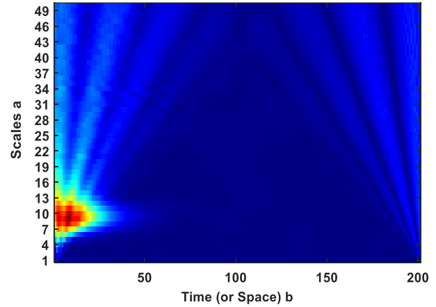
Figure 3: CWT of acceleration signal to the impulse input
