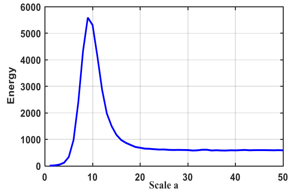
Figure 4: Energy distribution of Acceleration signal using CWT
