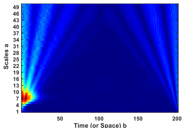
Figure 6: CWT of acceleration signal to the impulse input for faulty state 2
