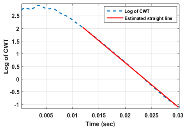
Figure 5: Cross-section for the logarithm of the CWT for scale a = 9 ( f_d = 180.5 Hz)
