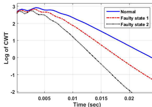
Figure 8: Comparison between Cross-section for the logarithm of the CWT in normal condition, faulty state 1 and faulty state 2
