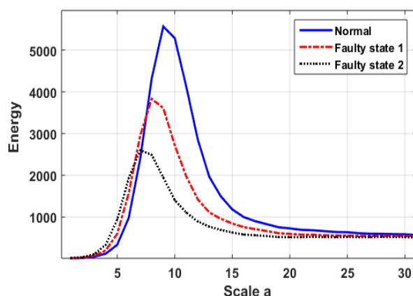
Figure 7: Comparison between energy distribution for acceleration of PREM in normal condition, faulty state 1 and faulty state 2 using CWT
