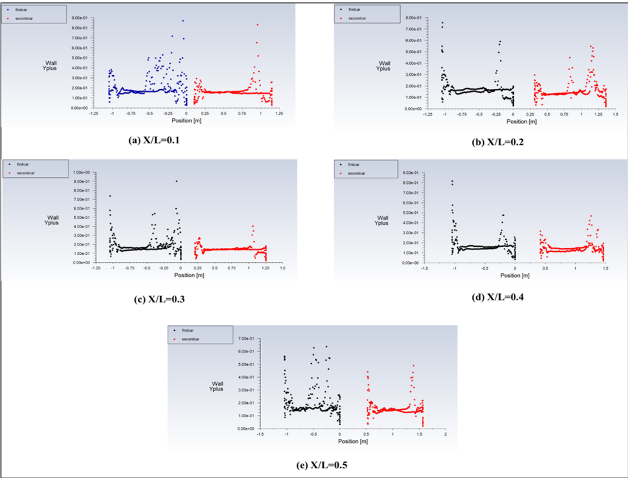
Figure 9. wall Y^+ distribution for two Ahmed bodies in tandem at different spacings ( X/L = 0.1-0.5 )
