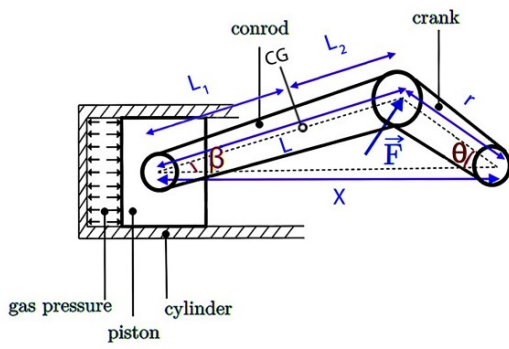
Figure 2: Dynamic model of the piston–crankshaft mechanism.
