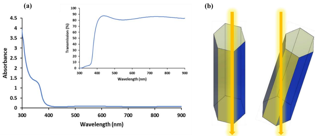
Figure 4: (a) Absorption spectra of the ZnO NRs. The inset shows the transmission spectra of the ZnO NRs. (b) the optical path traversing through nanorods
