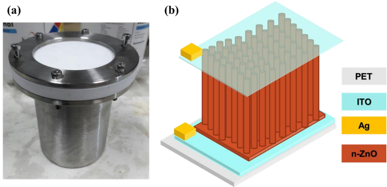
Figure 1: (a) stainless-steel Teflon-lined autoclave, (b) the schematic representation of the fabricated UV PD.
