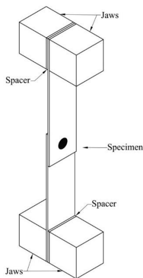
Figure 3: Schematics of tensile-shear test
