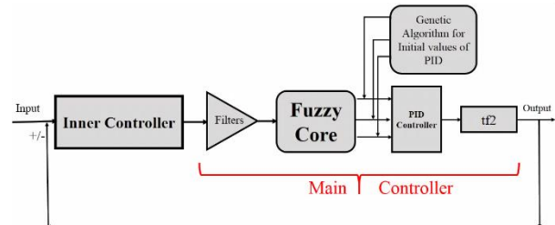
Figure8: Controller 2 scheme
