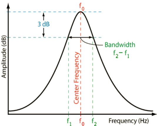
Fig 7.2 (a) Half wave band width technique
