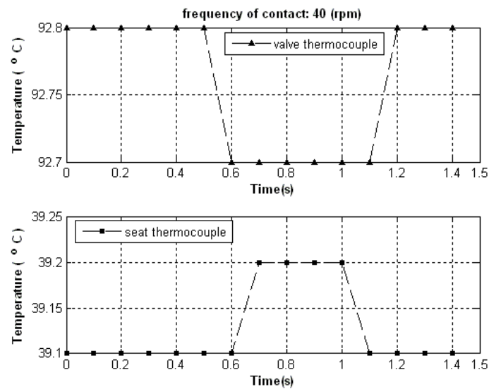
Fig5. Temperature distribution at the nearest thermocouples to the interface for the speed of 40 rpm
