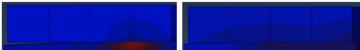
Fig9. contact situation between disk and pad after 1.6 sec in steel and FGM disks
