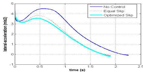
Figure10. Simulated lateral acceleration
