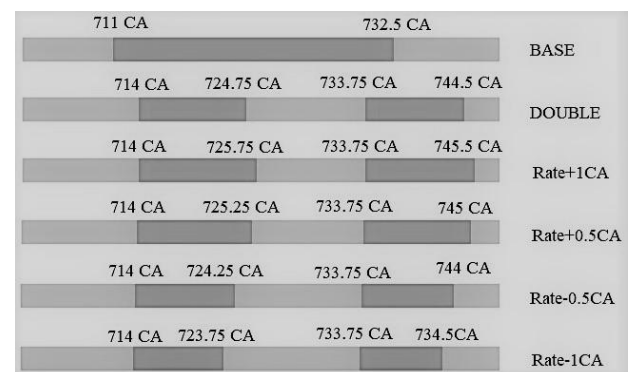
Figure 4. Schematic of injection schemes in this study
