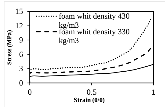
Figure 5. Stress-strain diagram of tubes filled by foams with densities of 230, 330, and 430 kg/m 3 resulted estimation method.
