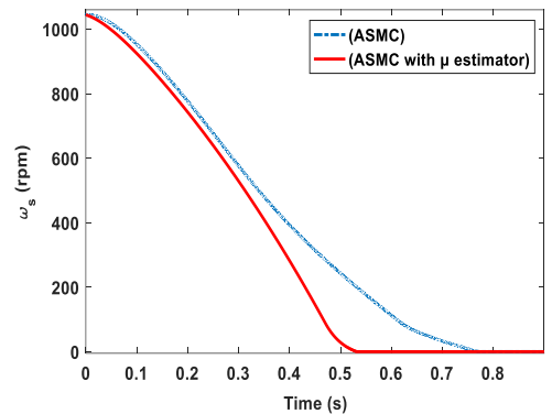
Figure 11: Slip speed during clutch engagement for the ASMC method in comparison with the ASMC system with \mu estimator in case of 20% uncertainties in the road friction coefficient (a): \omega_e and \omega_c of ASMC system, (b): \omega_e and \omega_c of ASMC system with \mu estimator, (C): Clutch slip speed
