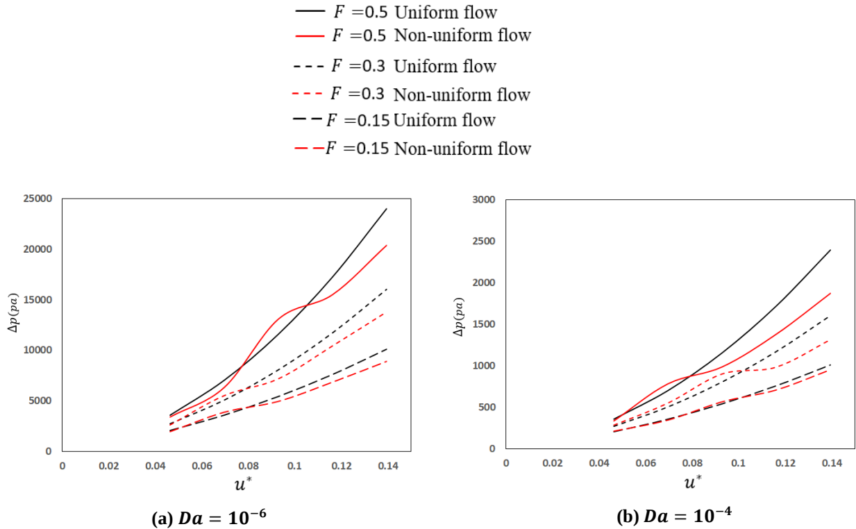
Figure 15: Effect of Forchheimer coefficient on pressure drop under uniform and non-uniform airflow, \phi = 0.97 and d_p = 0.01\text{mm} , (a) Da = 10^{-6} , (b) Da = 10^{-4} .
